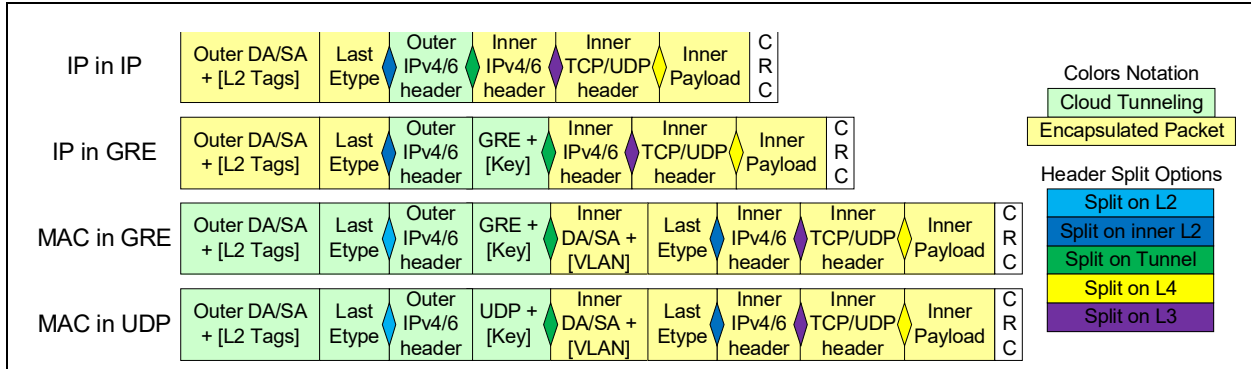
Figure 7-26. Tunneled packet formats
