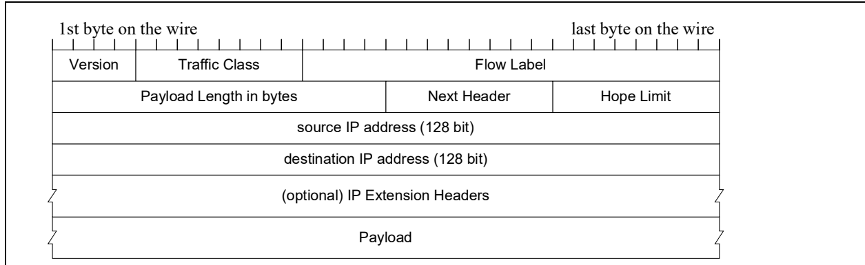
Figure 7-14. IPv6 datagram
